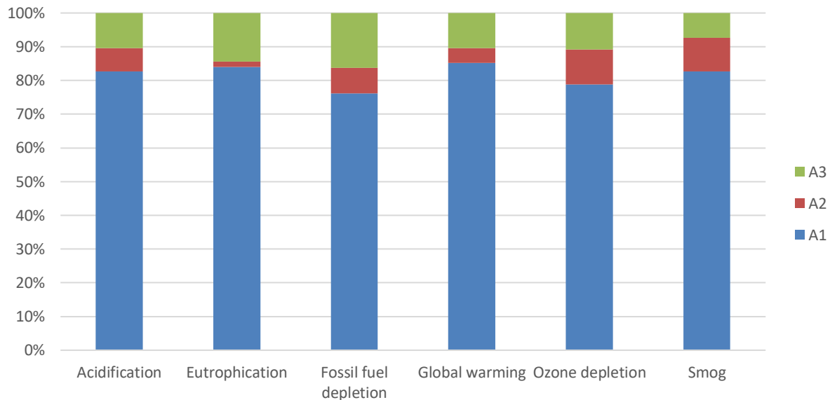
Figure 2. Contribution analysis for the Gerdau fabricated structural steel.
